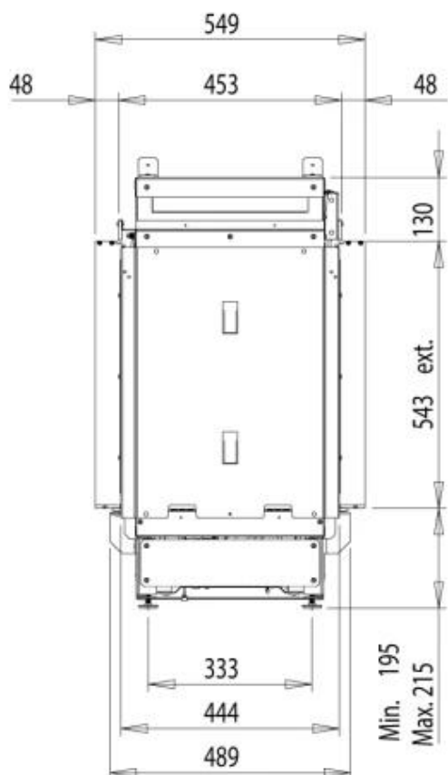
Dimensional Drawing e-Matrix heat 800x500 ST (MkII)
